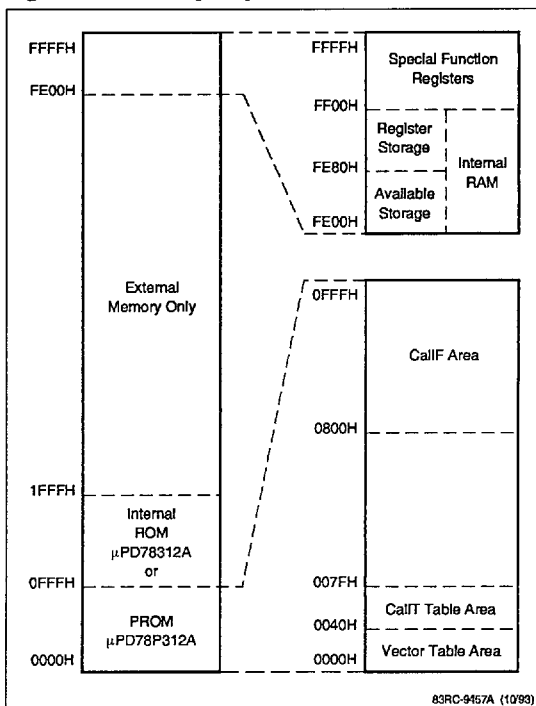
Figure 1. Memory Map
