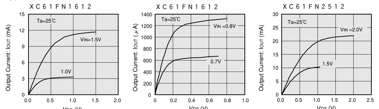
(4) N-CHANNEL DRIVER OUTPUT CURRENT vs. V_{DS}
