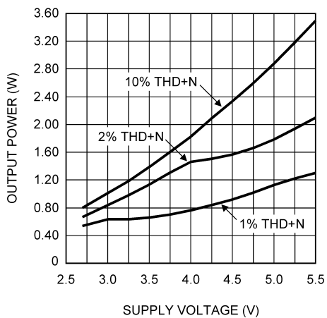
Output Power vs Supply Voltage R_L = 15\mu H + 4\Omega + 15\mu H , f = 1kHz
