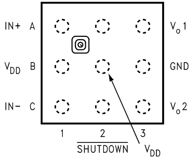
9 Bump micro SMD Package GAIN SELECT
