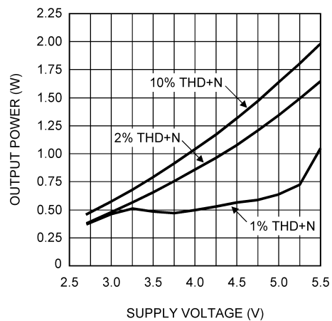
Output Power vs Supply Voltage R_L = 15\mu H + 8\Omega + 15\mu H , f = 1kHz
