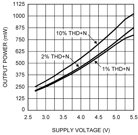
Output Power vs Supply Voltage R_L = 15\mu\text{H} + 16\Omega + 15\mu\text{H} , f = 1\text{kHz}
