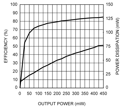
Efficiency and Power Dissipation vs Output Power V_{DD} = 3V , R_L = 15\mu H + 8\Omega + 15\mu H , f = 1kHz , THD < 1%
