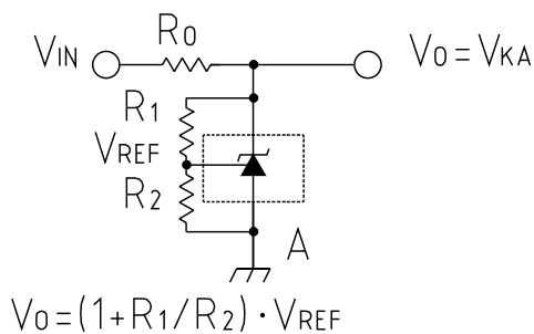
(2) V_{\text{KA}} \geq V_{\text{REF}} \quad V_0=V_{\text{KA}}=V_{\text{REF}}
