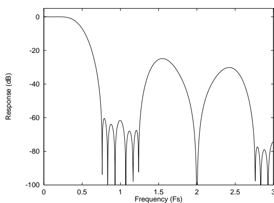
Figure 25 DAC Filter Frequency Response – Type 3
