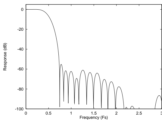
Figure 23 DAC Filter Frequency Response – Type 2
