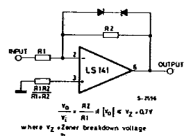
Fig. 28 - Clipping amplifier
