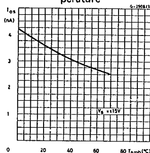
Fig. 24 - Input offset current vs. ambient temperature
