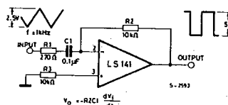
Fig. 30 - Simple differentiator
