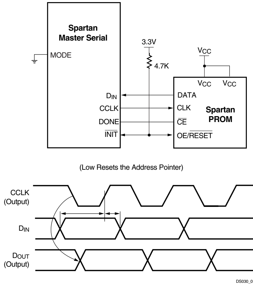
Figure 1: Master Serial Mode. The one-time-programmable Spartan PROM supports automatic loading of configuration programs. An early DONE inhibits the PROM data output one CCLK cycle before the Spartan FPGA I/Os become active.
