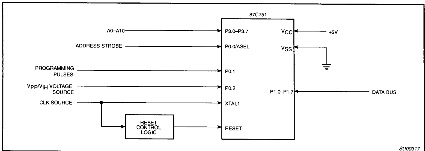
Figure 5. Programming Configuration
