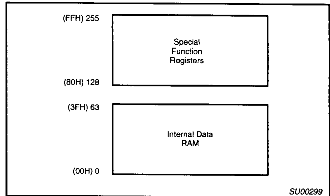
Figure 3. Memory Map
