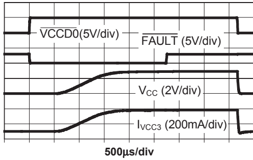
Turn-ON/OFF Response with 10Ω, 1μF load ( \overline{\text{VCCD1}} = 0\text{V} )
