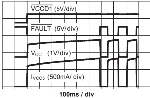
Thermal Shutdown Response ( \overline{\text{VCCD0}} = 0\text{V} )
