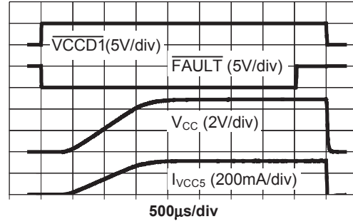
Turn-ON/OFF Response with 15Ω, 1μF load ( \overline{\text{VCCD0}} = 0\text{V} )
