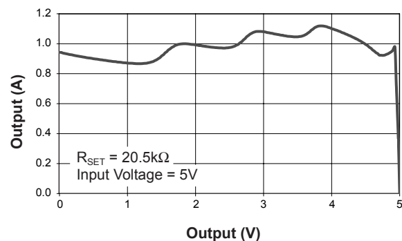
Current Limit ( V_{IN} = 5.0V )
