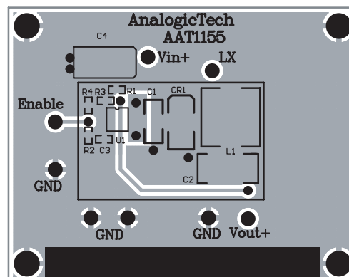
Figure 7. Evaluation Board Bottom Side
