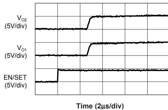
Turn-On Characteristic V_{IN}=5V , R_{L1}=R_{L2}=50\Omega , C_{O1}=C_{O2}=0.1\mu F
