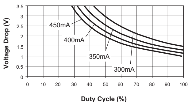
Device Duty Cycle vs. V_{DROP} V_{OUT} = 1.5\text{V} @ 85^\circ\text{C}
