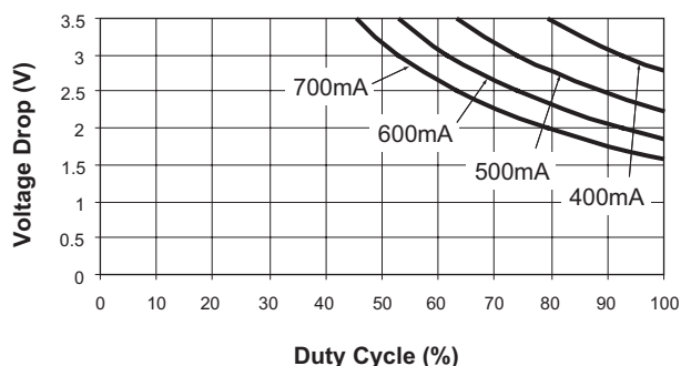
Device Duty Cycle vs. V_{DROP} V_{OUT} = 1.5\text{V} @ 25^\circ\text{C}
