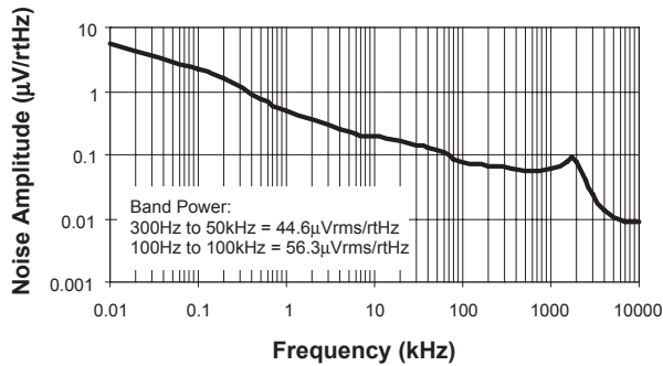
AAT3258 Self Noise C_{\text{OUT}} = 10\mu\text{F} (ceramic)
