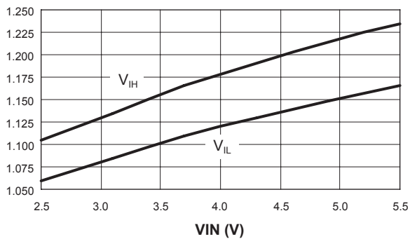
LDO SHDN V_{\text{IH}} and V_{\text{IL}} vs. V_{\text{IN}}
