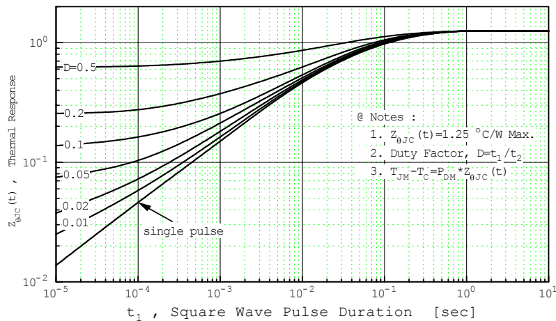
Figure 11. Thermal Response
