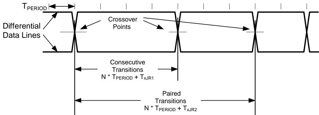
Figure 23-5. Differential Data Jitter
