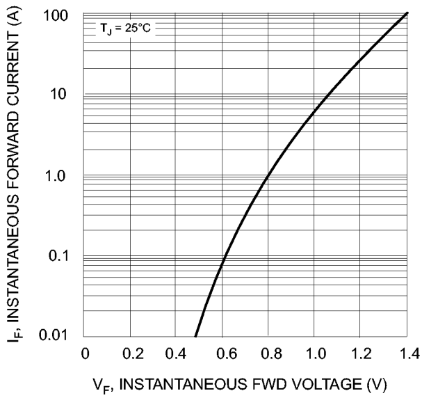
Fig. 3, Typ. Instantaneous Forward Characteristics
