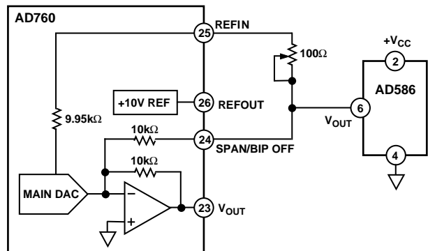
Figure 7. Using the AD760 with the AD586 5 V Reference
