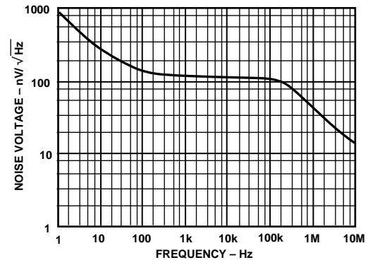
Figure 13. DAC Output Noise Voltage Spectral Density
