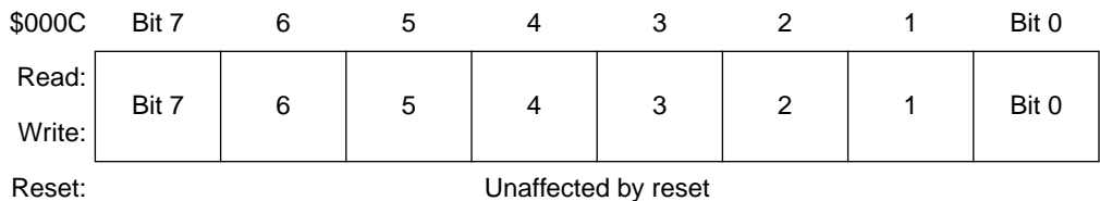
Figure 66. SIOP Data Register (SDR)
