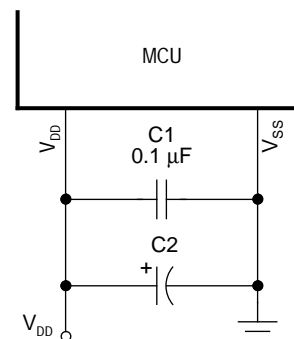
Figure 3. Bypassing Recommendation
