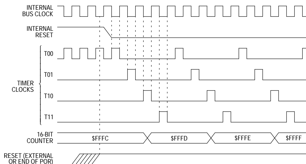
Figure 47. Timer Reset Timing
