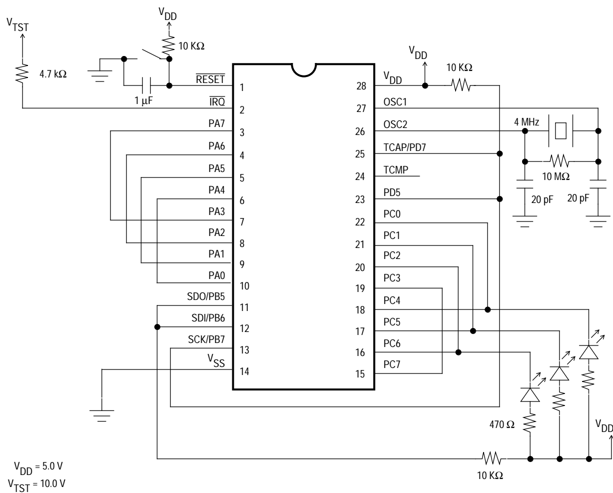
Figure 10. Self-Check Circuit
