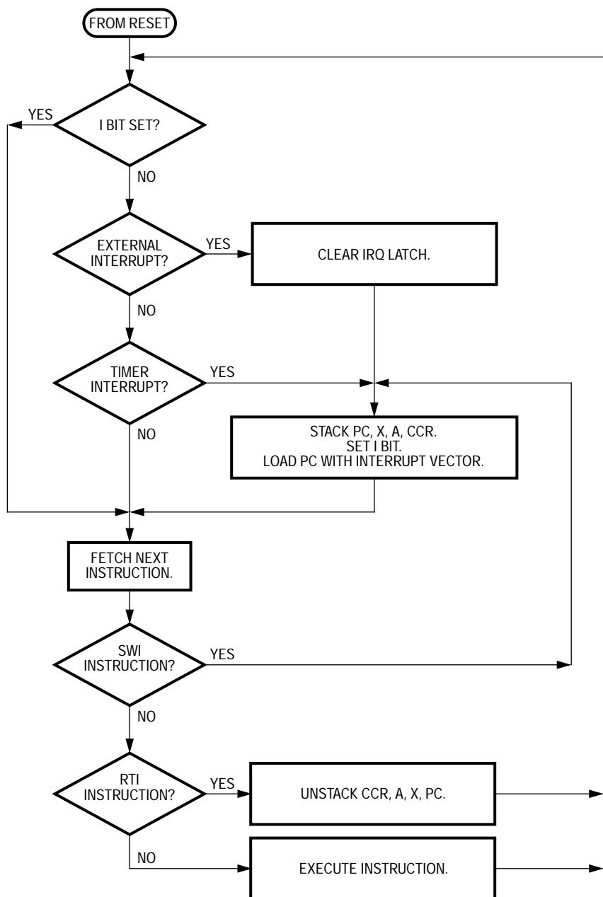
Figure 23. Interrupt Flowchart
