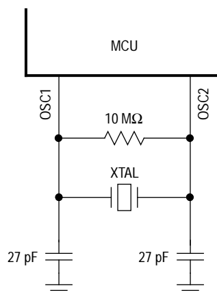
Figure 4. Crystal Connections
