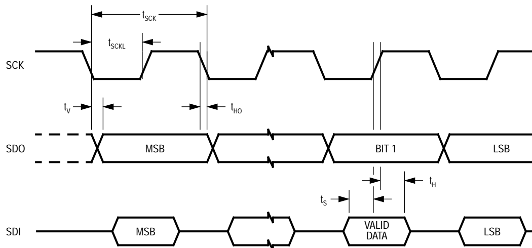
Figure 63. SIOF Timing
