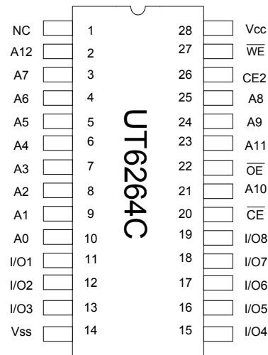
PDIP/SOP
