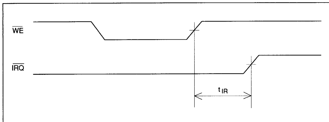
Figure 16 WE and IRQ Timing
