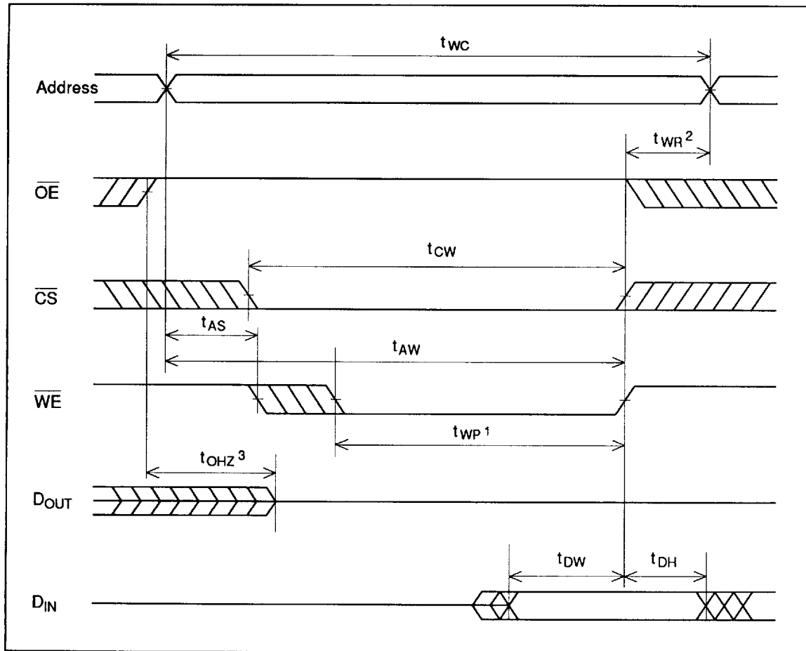
Figure 13 Write Cycle Timing 1
