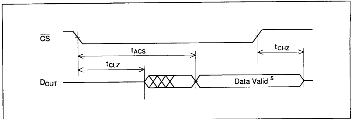
Figure 12 Read Cycle Timing
