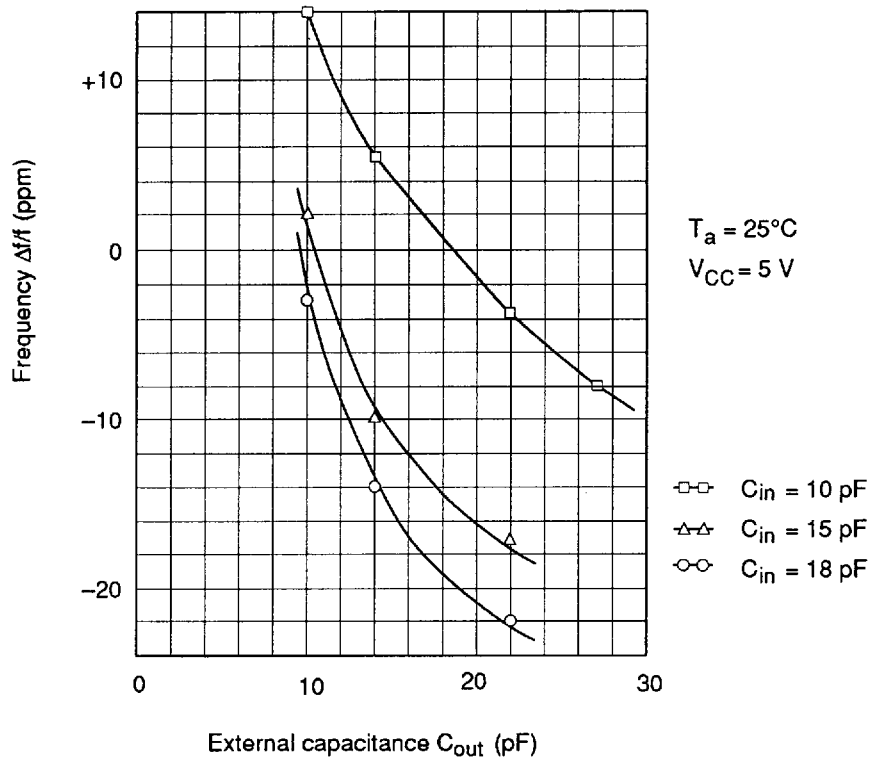
Figure 27 Frequency vs. External Capacitance
