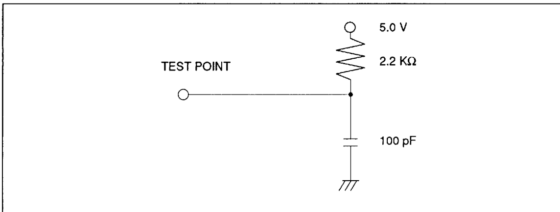
Figure 21 Load B (IRQ)
