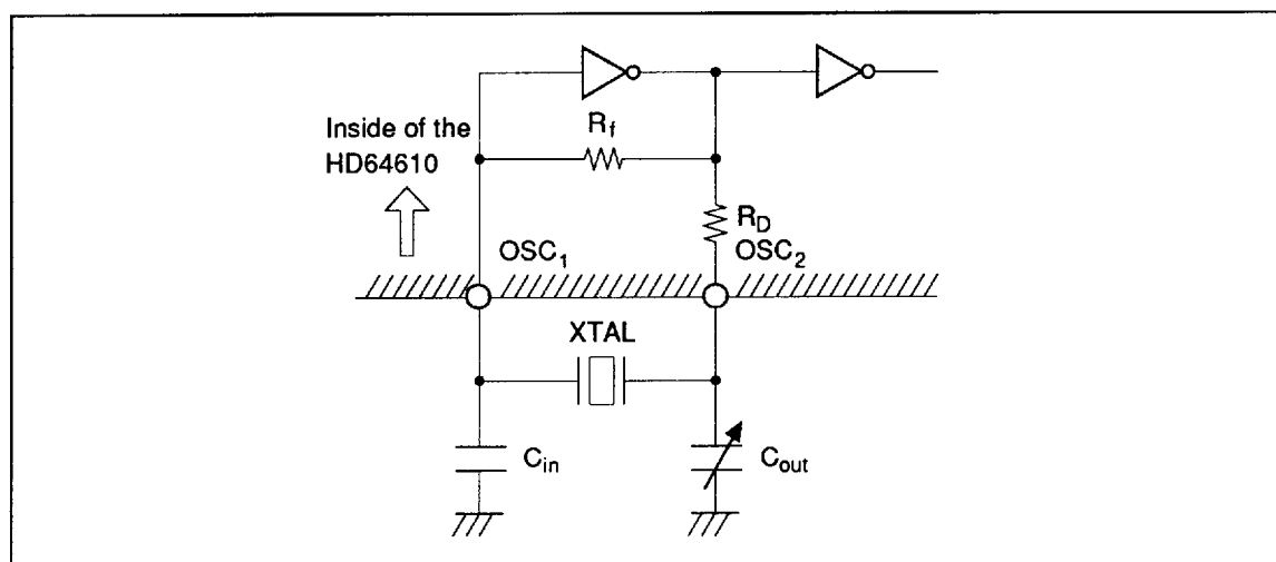
Figure 7 Crystal Oscillator Circuit Example
