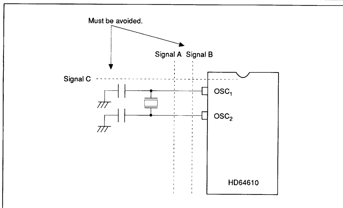
Figure 8 Signal Layout to be Avoided
