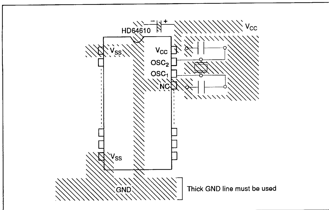
Figure 9 Board Design Example
