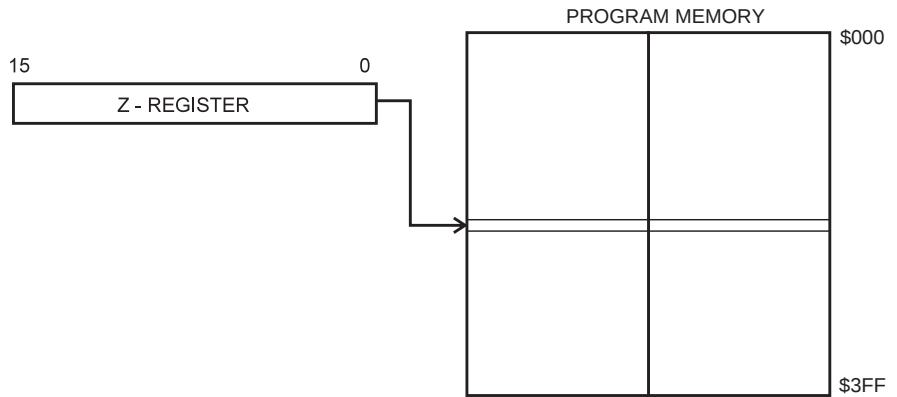
Figure 15. 间接程序存储器寻址
