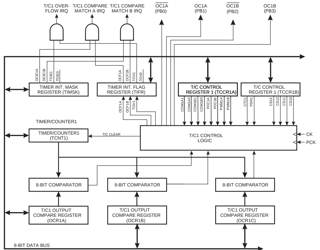
Figure 35. T/C1 方框图
