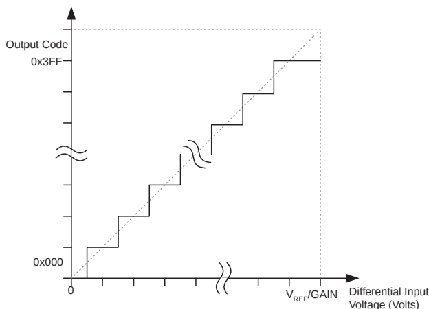
Figure 51. 差分测量范围
