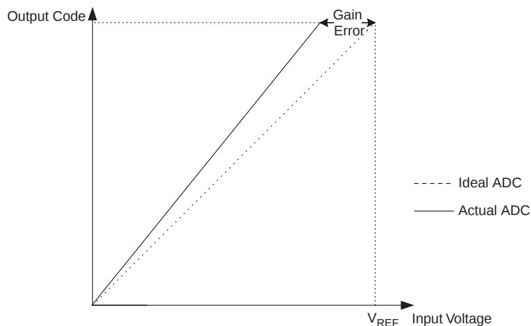
Figure 108. 增益误差
