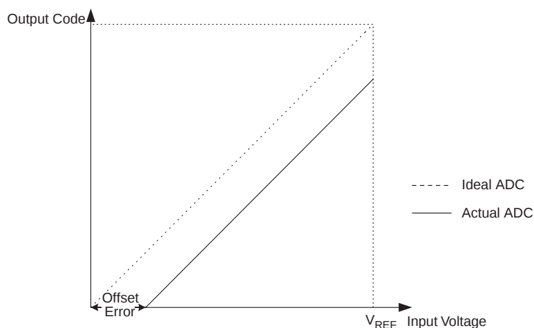
Figure 107. 偏移误差
