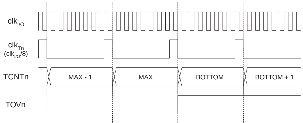
Figure 61. T/C 时序图，预分频器为 f_{clk\_I/O}/8
