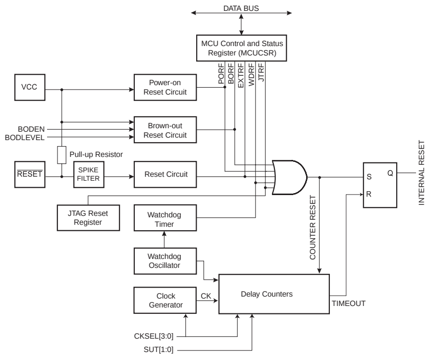
Figure 15. 复位逻辑
