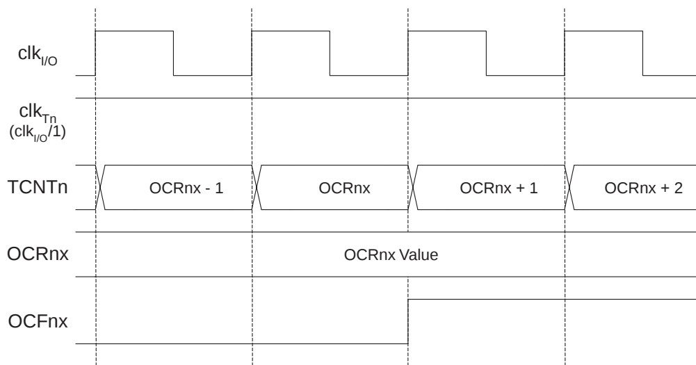
Figure 49. T/C 时序图，OCF1x 置位，无预分频器
