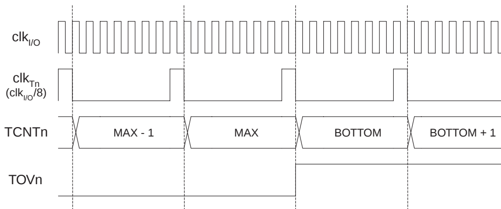
Figure 35. T/C 时序图，预分频器为 f_{clk\_I/O}/8
