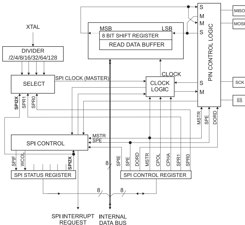
Figure 65. SPI 方框图 (1)
