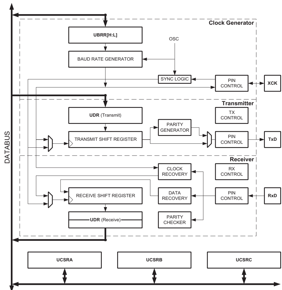
Figure 69. USART 方框图 (1)
