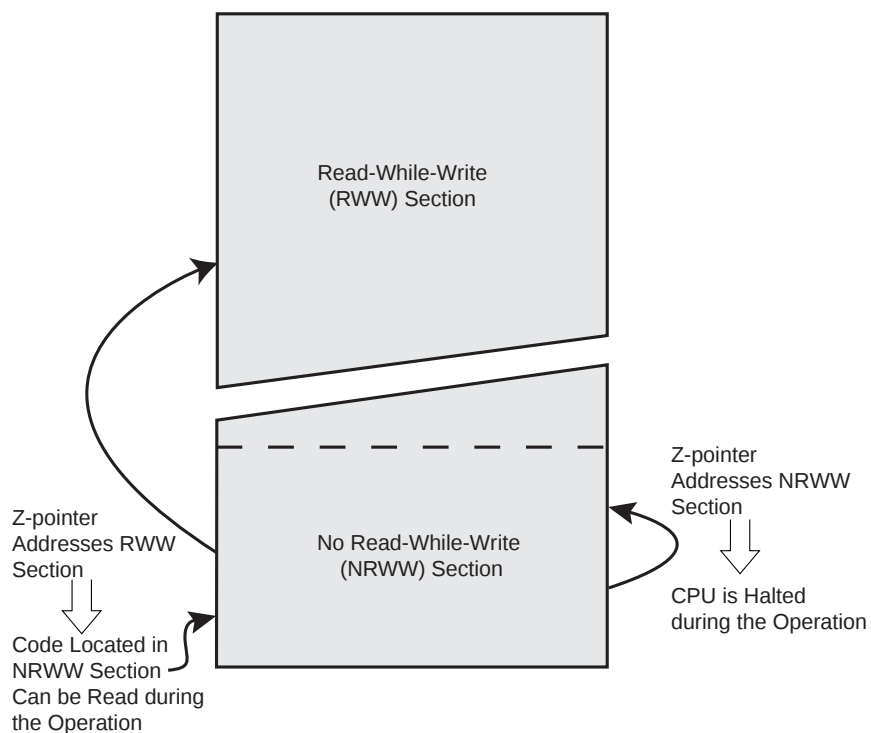
Figure 124. RWW 与 NRWW
