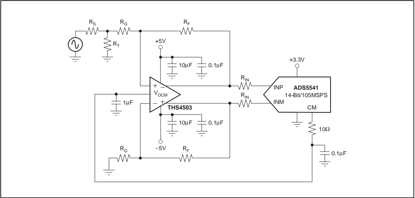
Figure 7. Using the THS4503 with the ADS5541
