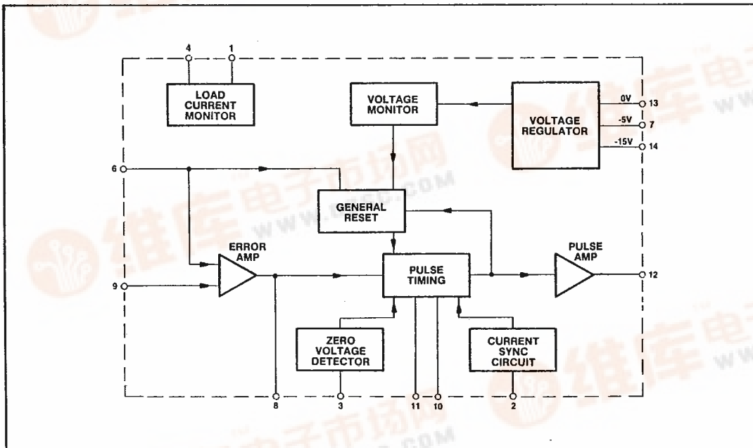
Fig.2 Block diagram
