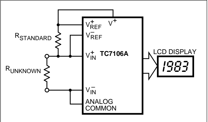
Figure 17. Low Parts Count Ratiometric Resistance Measurement
