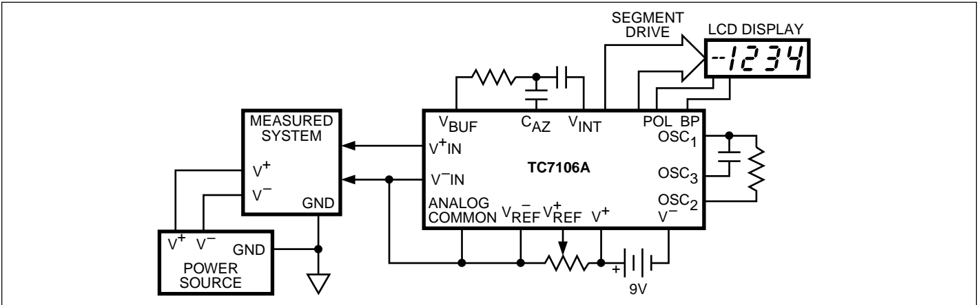
Figure 8. Common-Mode Voltage Removed in Battery Operation with V^- to Analog Common
