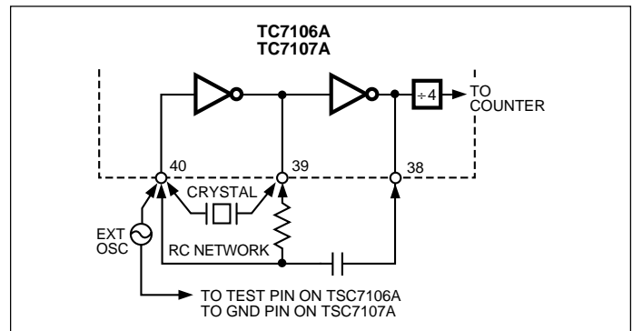
Figure 6. Clock Circuits
