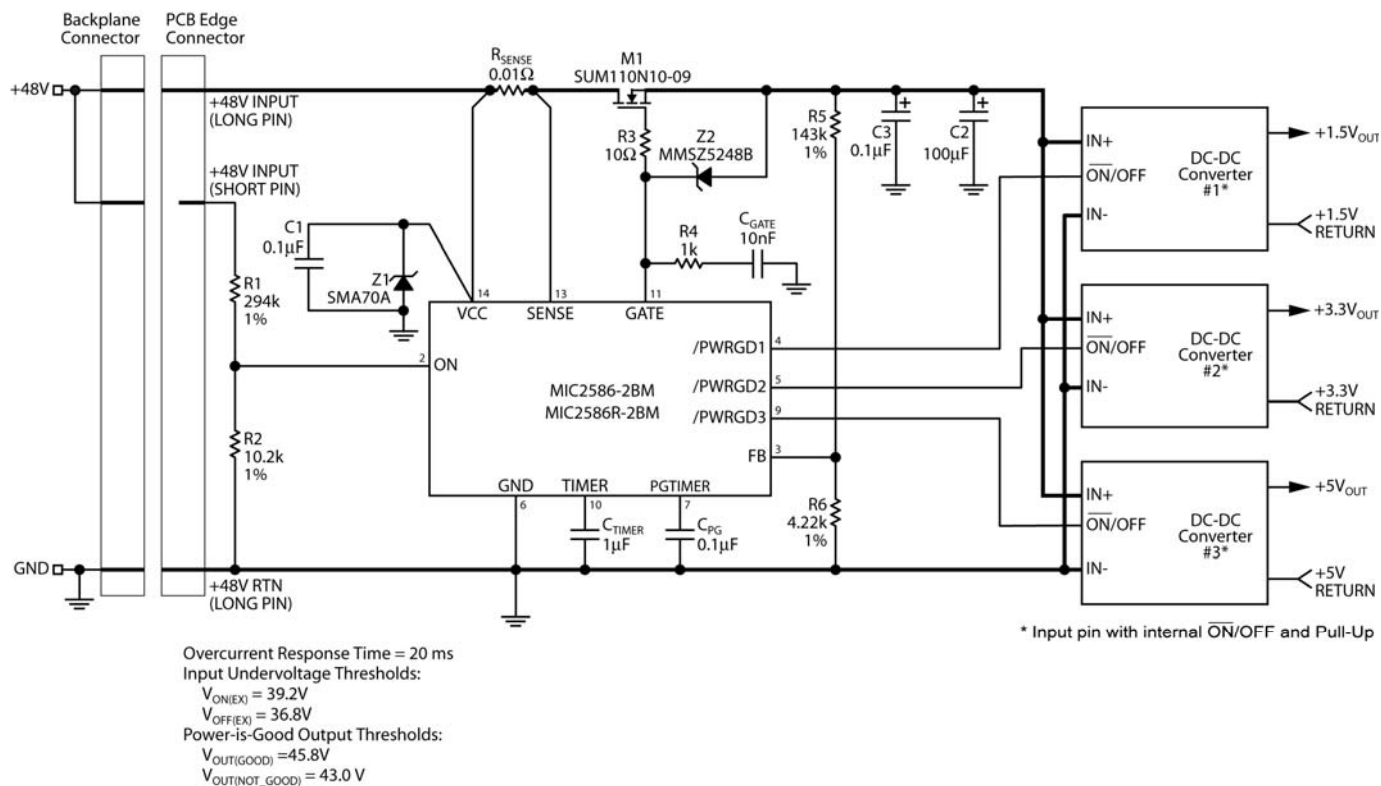
MIC2586/86R Typical Application Circuit
