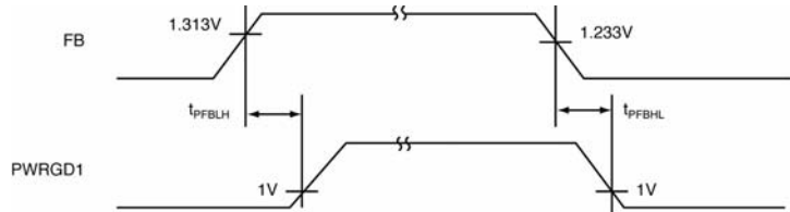
Figure 3. MIC2586/86R-1 FB to PWRGD1 Timing
