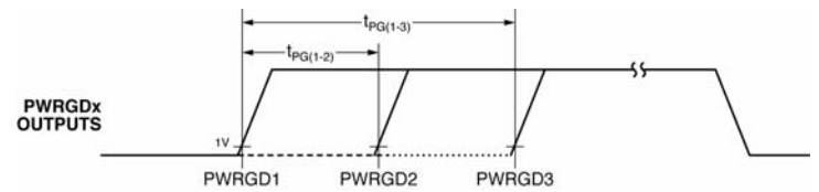
Figure 5. MIC2586/86R-1 Multiple PWRGDx Timing
