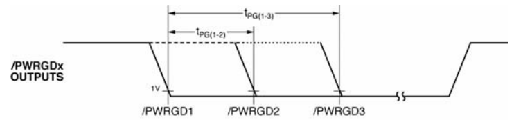
Figure 6. MIC2586/86R-2 Multiple /PWRGDx Timing
