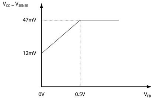
Figure 1. Foldback Current Limit Transfer Characteristic
