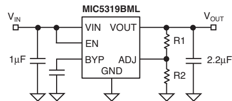
Figure 1. Adjustable Voltage Application
