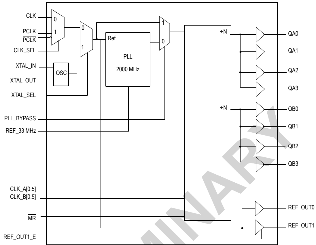
Figure 1. MPC9855 Logic Diagram
