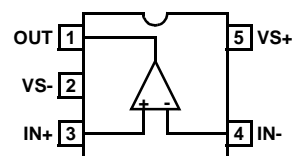
EL5135 (5-PIN SOT-23) TOP VIEW
