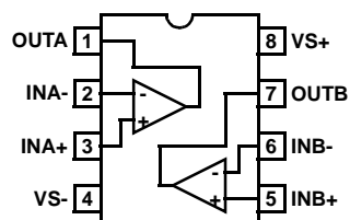
EL5235 (8-PIN SO) TOP VIEW
