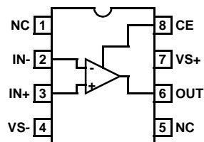
EL5134 (8-PIN SO) TOP VIEW
