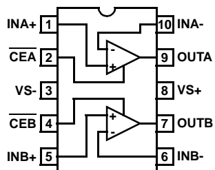
EL5234 (10-PIN MSOP) TOP VIEW
