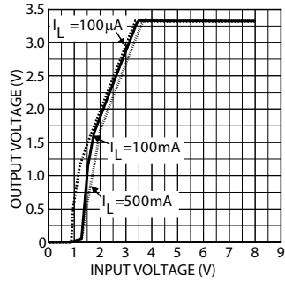
Dropout Characteristics
