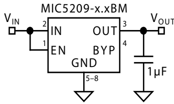
Figure 1. Low-Noise Fixed Voltage Regulator
