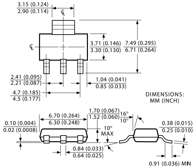
SOT-223 (S)
