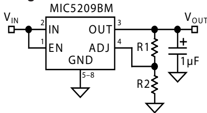
Figure 3. Low-Noise Adjustable Voltage Regulator
