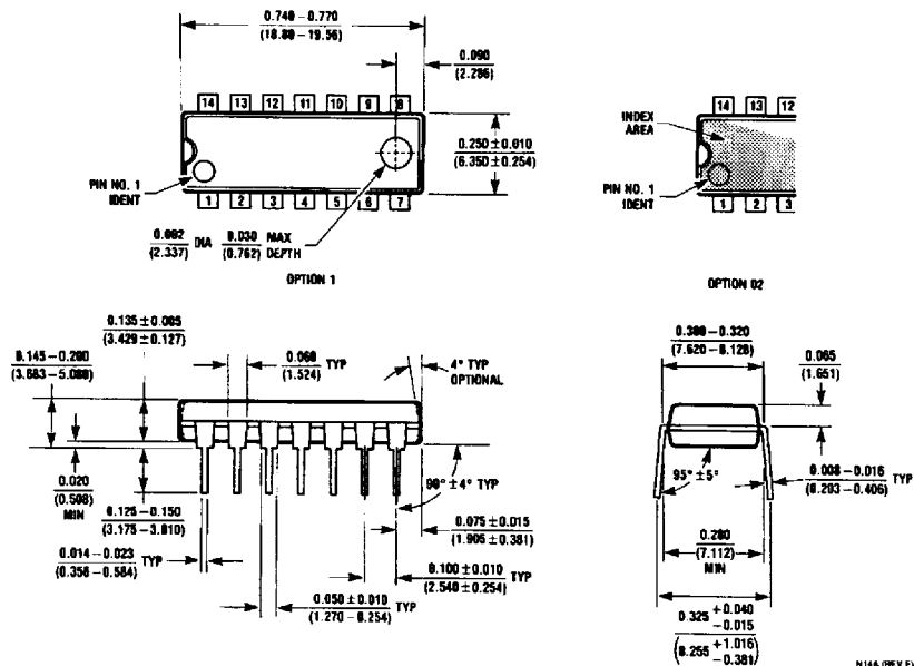
14-Lead Molded Dual-In-Line Package (N) Order Number DM7490AN or DM7493AN NS Package Number N14A
