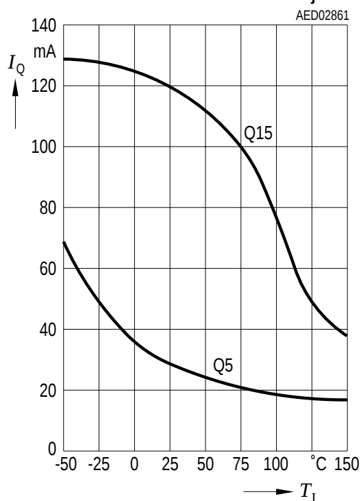
Output Current Limit I_{Q5} and I_{Q15} versus Junction Temperature T_j
