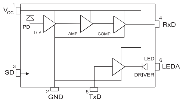
Figure 1. IrMC Transceiver Block Diagram
