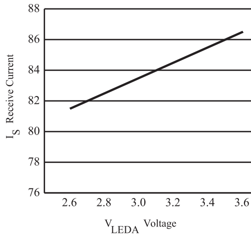
Figure 7. Receive Current Versus Supply Voltage ( T_a=25\text{ }^\circ\text{C} )
