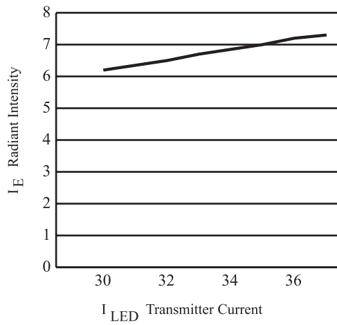
Figure 6. Radiant Intensity Versus Transmitter Current (Ta=25 °C)
