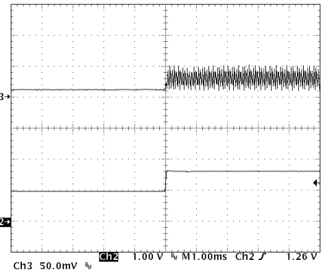
Upper Trace: Output Voltage Ripple, 50 mV/Division Lower Trace: Battery Voltage, V_{IN} , 1.0 V/Division ( V_{IN} = 1.0\text{ V to } 1.6\text{ V} ; L = 5.6\text{ }\mu\text{H} , C_{OUT} = 22\text{ }\mu\text{F} , I_{LOAD} = 50\text{ mA} )
