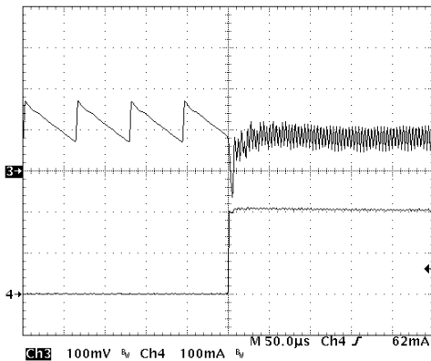
Upper Trace: Output Voltage Ripple, 100 mV/Division Lower Trace: Load Current, I_{LOAD} , 100 mA/Division ( V_{OUT} = 3.3\text{ V} , I_{LOAD} = 10\text{ mA to } 200\text{ mA} ; L = 5.6\text{ }\mu\text{H} , C_{OUT} = 22\text{ }\mu\text{F} )
