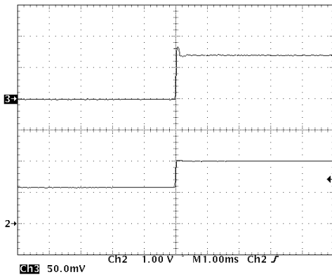
Upper Trace: Output Voltage Ripple, 50 mV/Division Lower Trace: Battery Voltage, V_{IN} , 1.0 V/Division ( V_{IN} = 1.2\text{ V to } 2.0\text{ V} ; L = 5.6\text{ }\mu\text{H} , C_{OUT} = 22\text{ }\mu\text{F} , I_{LOAD} = 50\text{ mA} )
