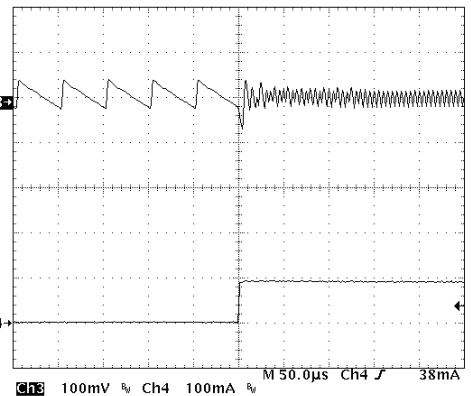
Upper Trace: Output Voltage Ripple, 100 mV/Division Lower Trace: Load Current, I_{LOAD} , 100 mA/Division ( V_{OUT} = 1.8\text{ V} , I_{LOAD} = 10\text{ mA to } 100\text{ mA} ; L = 5.6\text{ }\mu\text{H} , C_{OUT} = 22\text{ }\mu\text{F} )
