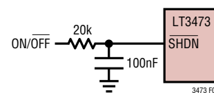
Figure 4. Soft-Start Circuitry
