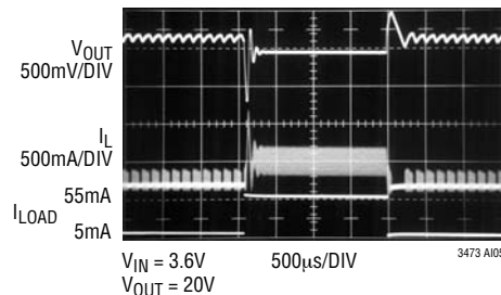
Transient Response
