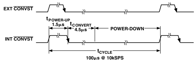
Figure 9. Automatic Power-Down
