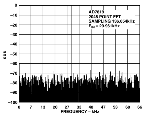
Figure 11. SNR
