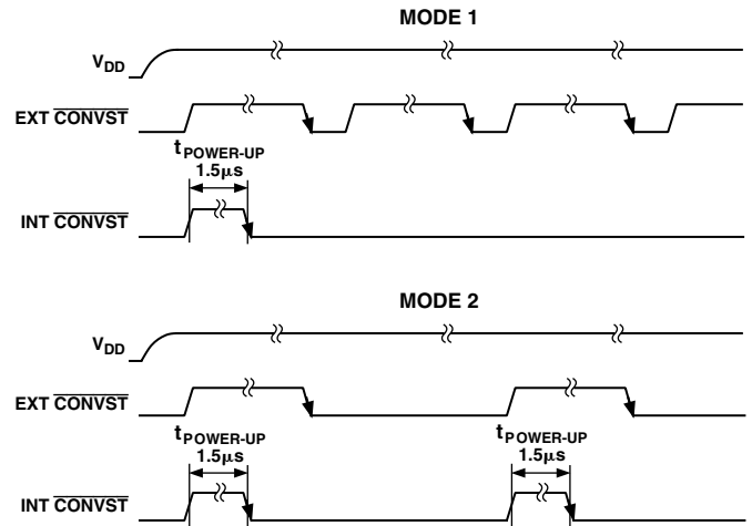
Figure 8. Power-Up Times
