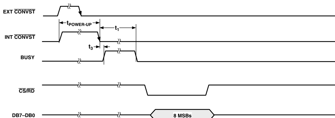
Figure 14. Mode 2 Operation
