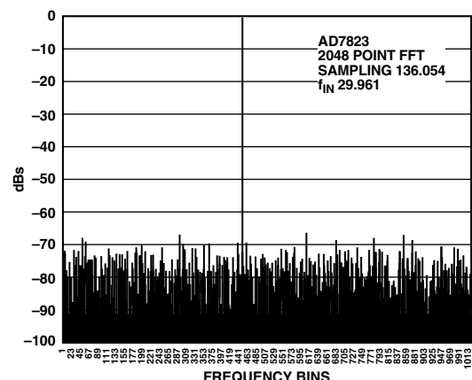
Figure 3. Frequency Spectrum
