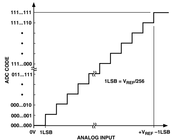
Figure 11. Transfer Characteristic
