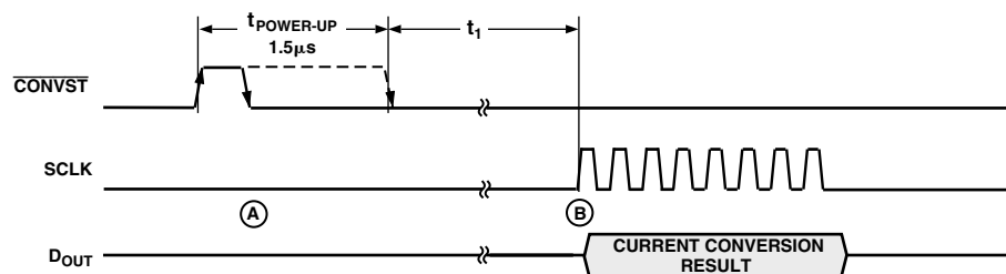
Figure 15. Mode 2 Operation Timing
