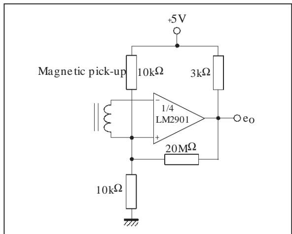
TRANSDUCER AMPLIFIER
