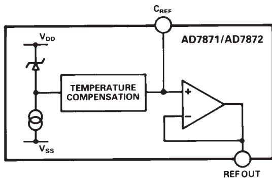
Figure 3. Reference Circuit
