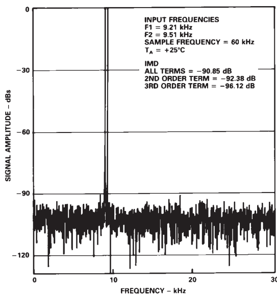
Figure 16. IMD Plot
