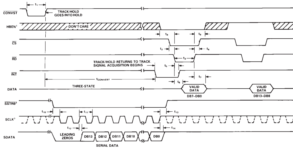
Figure 10. Mode 1 Timing Diagram, Byte or Serial Read
