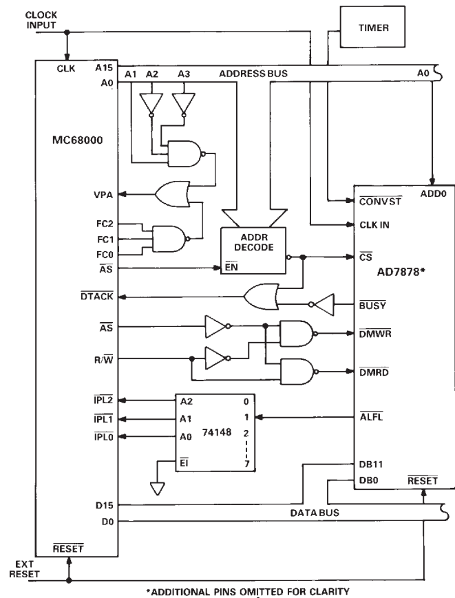
Figure 21. AD7878-MC68000 Interface
