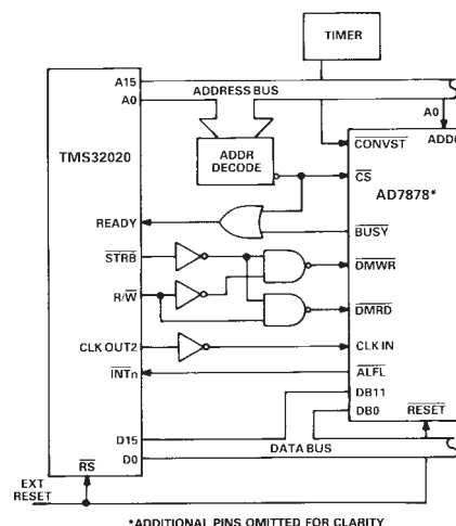
Figure 19. AD7878-TMS32020 Interface
