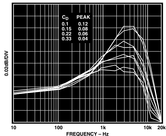
Figure 11. Jitter Transfer vs. C
