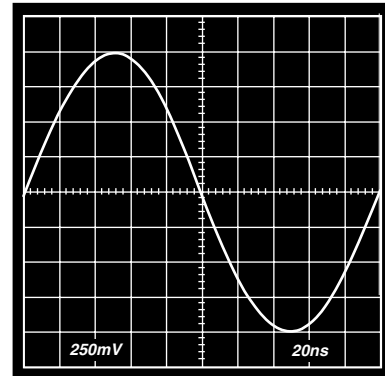
TPC 24. Sine Response; G = +2 , V_S = \pm 2.5 V^*
