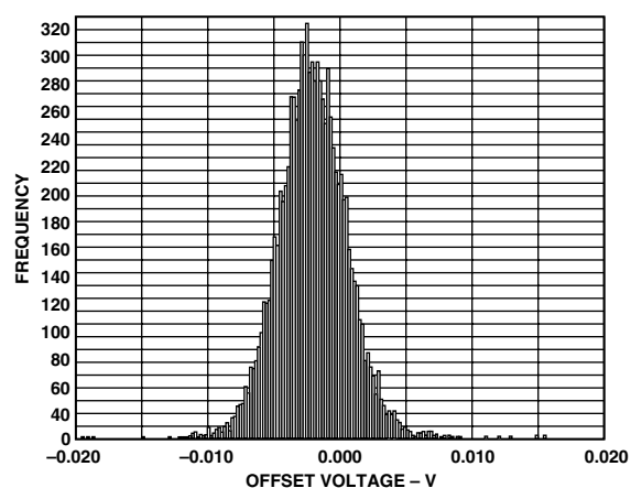
TPC 35. AD8109 Offset Voltage Distribution (RTI)
