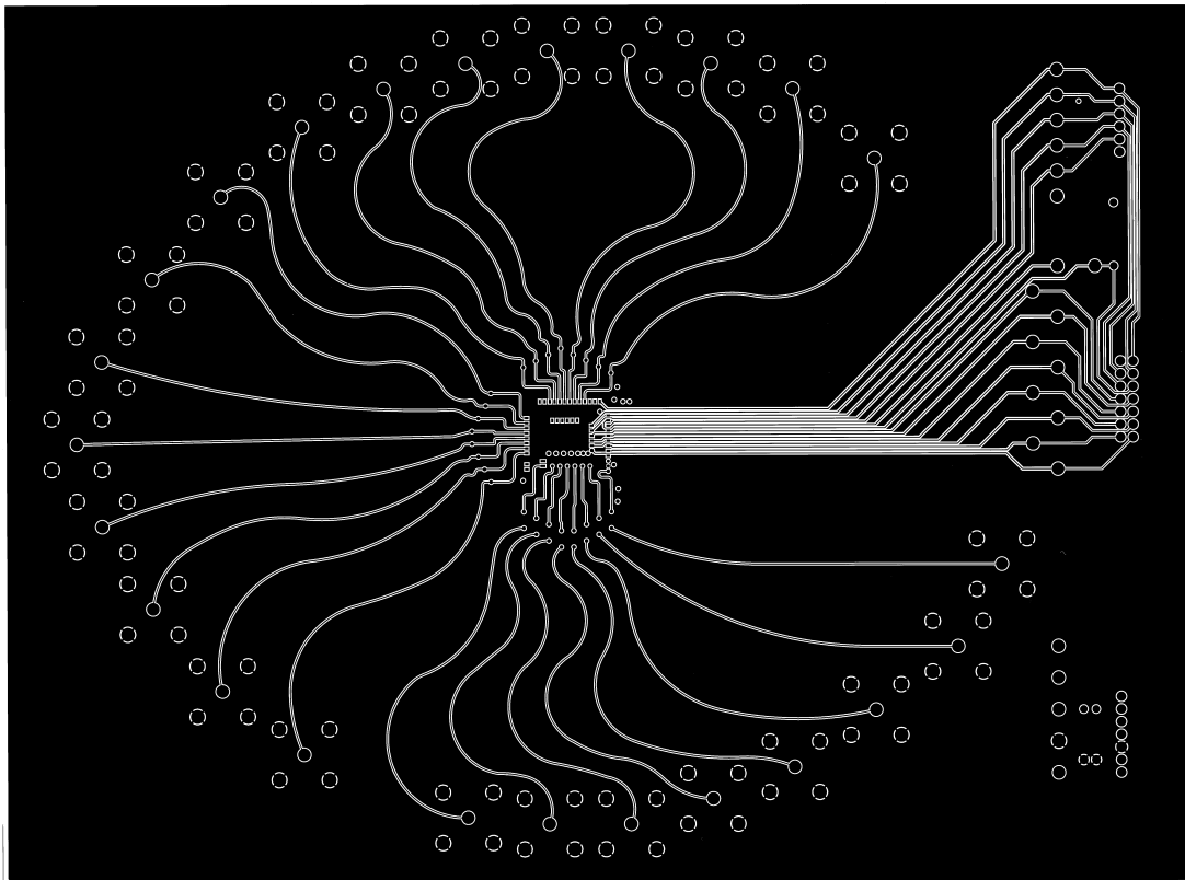
Figure 13. Board Layout (Signal Layer)
