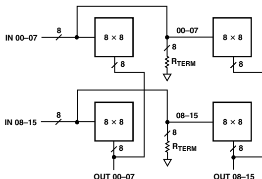
Figure 7. 16 \times 16 Crosspoint Array Using Four AD8108s or AD8109s
