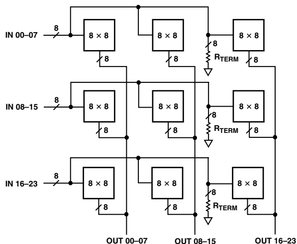
Figure 8. 24 \times 24 Crosspoint Array Using Nine AD8108s or AD8109s
