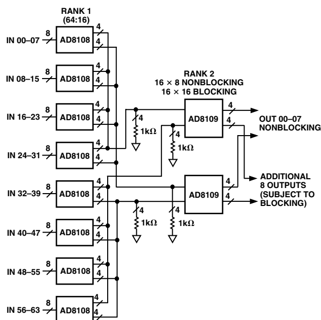
Figure 9. Nonblocking 64 \times 8 Array with Gain-of-Two ( 64 \times 16 Blocking)
