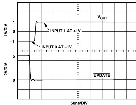
TPC 28. AD8108 Switching Time
