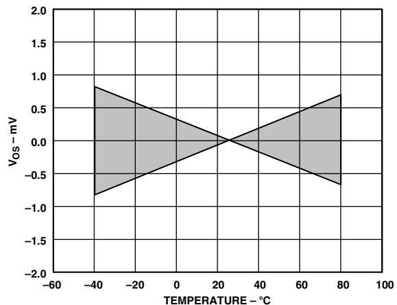
TPC 30. AD8108 Offset Voltage Drift vs. Temperature (Normalized at 25°C)
