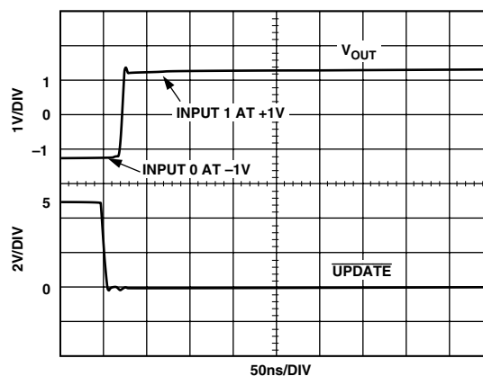
TPC 34. AD8109 Switching Time
