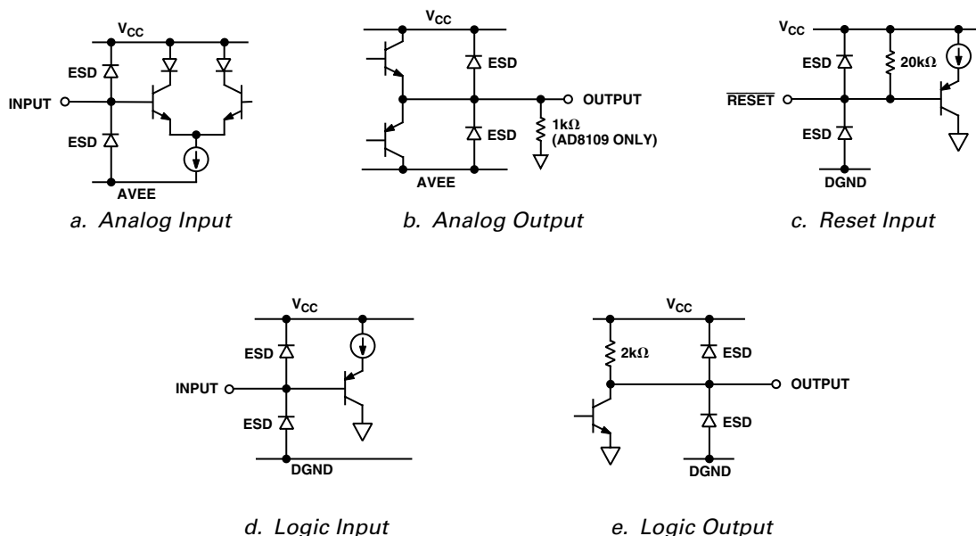
Figure 5. I/O Schematics
