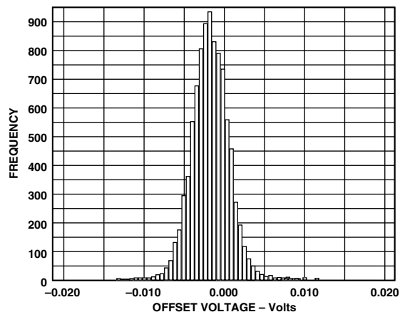
TPC 29. AD8108 Offset Voltage Distribution
