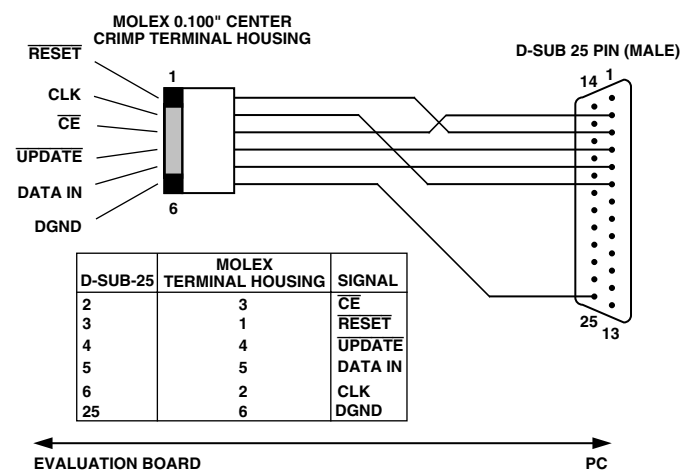
Figure 17. Evaluation Board-PC Connection Cable
