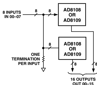
Figure 6. 8 \times 16 Crosspoint Array Using Two AD8108s (Unity Gain) or Two AD8109s (Gain-of-Two)
