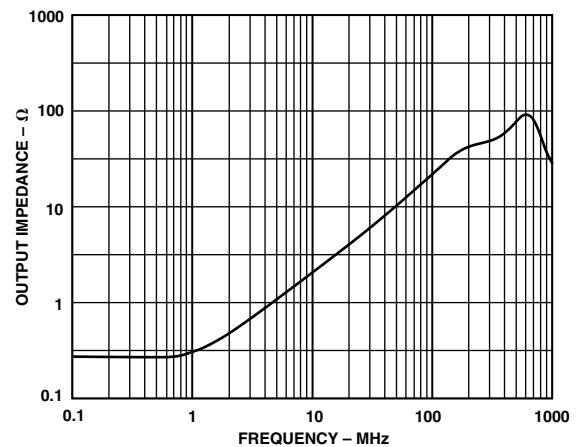
TPC 17. AD8115 Output Impedance, Enabled vs. Frequency
