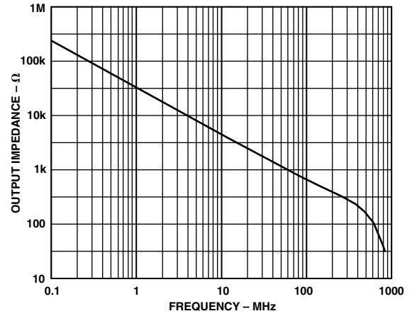
TPC 18. AD8115 Output Impedance, Disabled vs. Frequency
