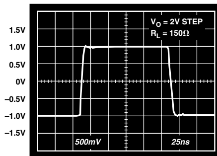
TPC 26. AD8114 Pulse Response, Large Signal
