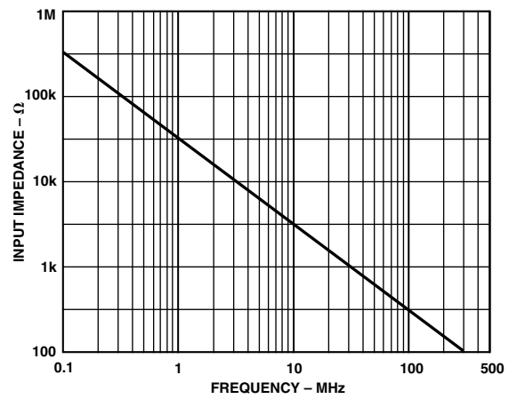
TPC 16. AD8115 Input Impedance vs. Frequency
