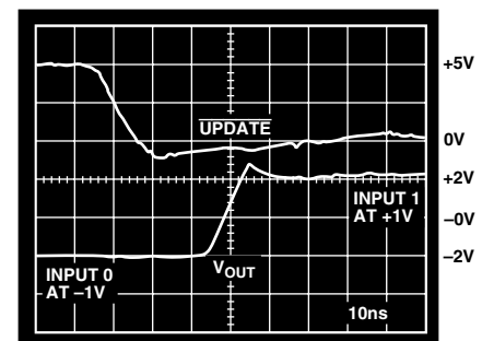
TPC 30. AD8115 Switching Time
