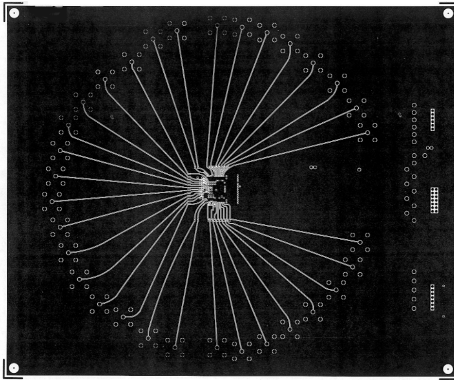
Figure 11. Board Layout (Signal Layer)
