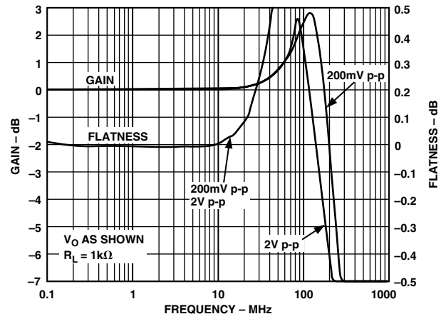
TPC 5. AD8115 Frequency Response; R_L = 1 \text{ k}\Omega
