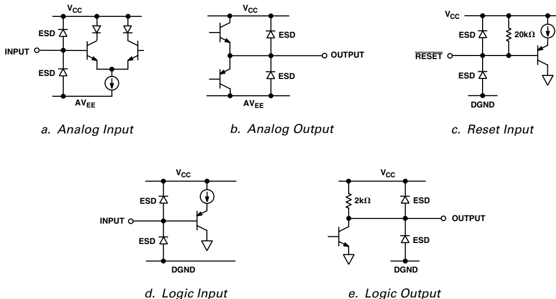
Figure 5. I/O Schematics
