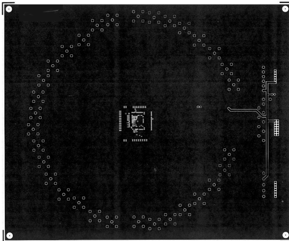
Figure 12. Board Layout (Ground Plane)
