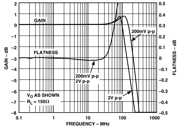
TPC 4. AD8115 Frequency Response; R_L = 150 \Omega
