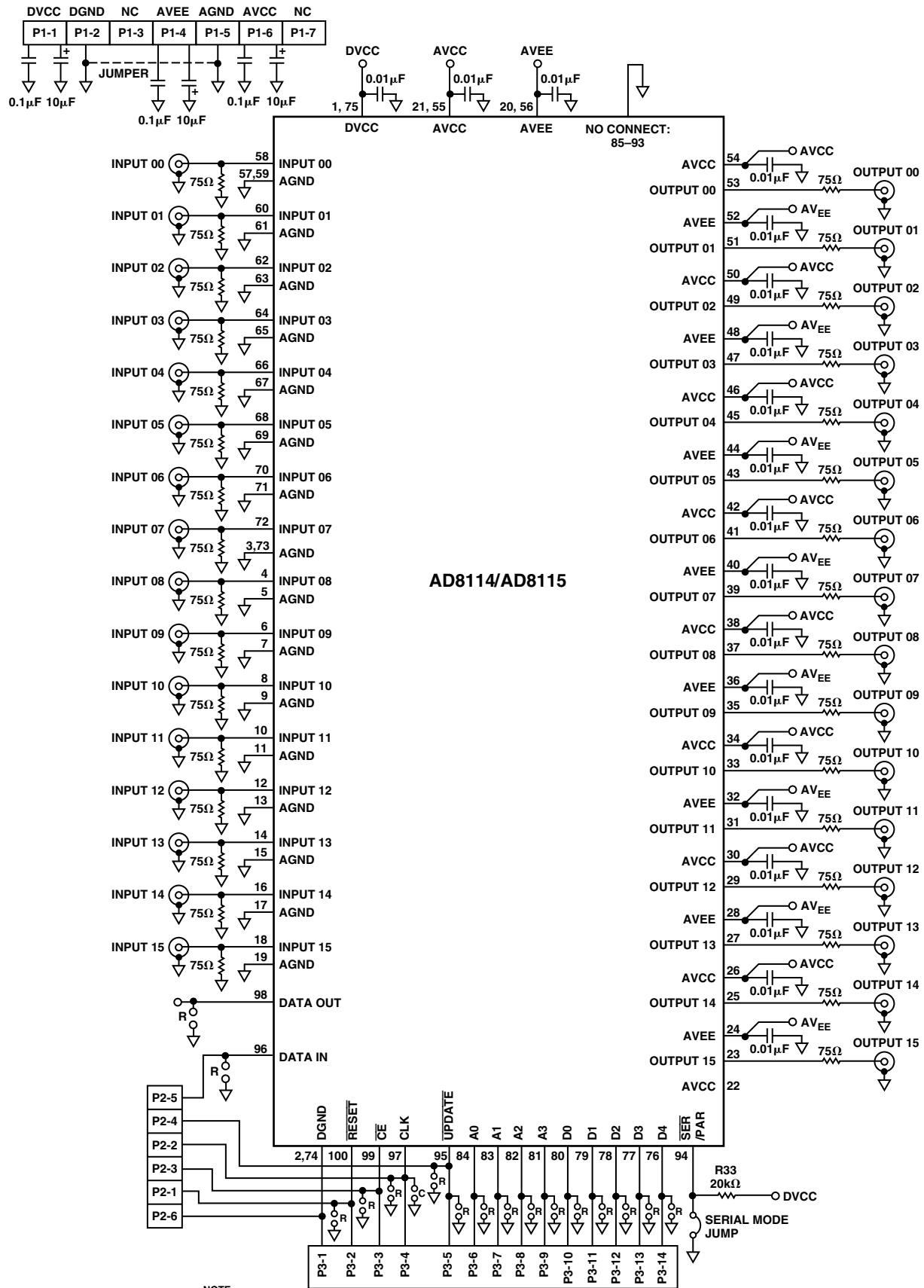
Figure 8. Evaluation Board Schematic
