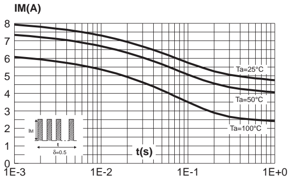
Fig. 3-1: Non repetitive surge peak forward current versus overload duration (maximum values) (SMB).
