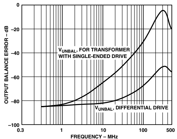
Figure 5. Output Balance Error for Circuits of Figures 3 and 4
