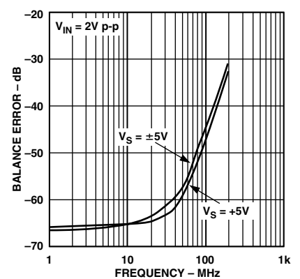
TPC 27. Output Balance Error vs. Frequency
