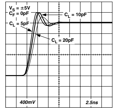
TPC 24. Large Signal Transient Response for Various Cap Loads
