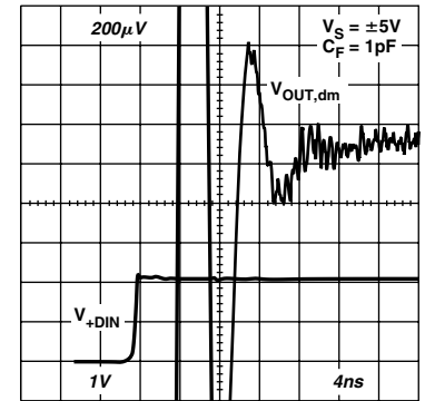
TPC 21. Settling Time
