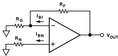
Figure 42. Output Offset Voltage
