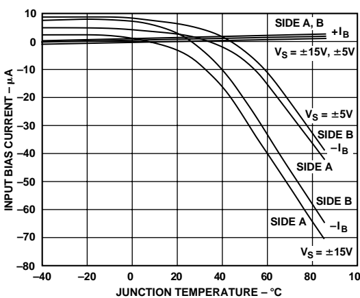
Figure 6. Input Bias Current vs. Temperature
