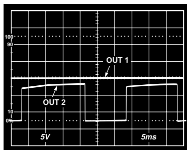
Figure 47. OUT1 Shorted to Ground, Square Wave Is OUT2, R_F = 1\text{ k}\Omega , R_G = 222\text{ }\Omega
