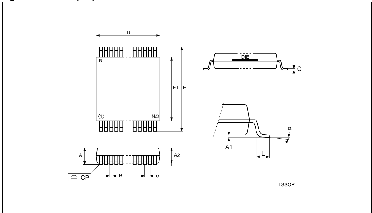
Figure 13. TSSOP8 (DW)
