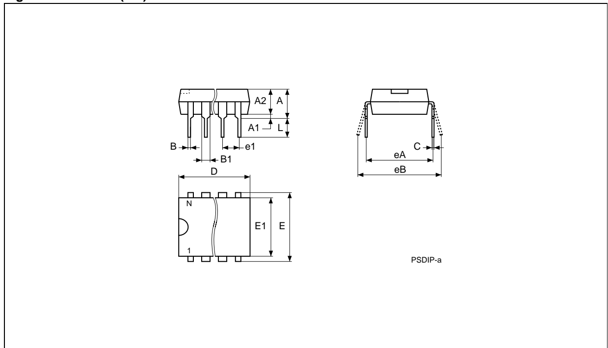
Figure 11. PSDIP8 (BN)
