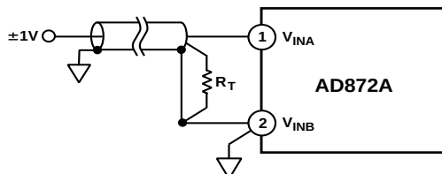
Figure 14. AD872A Single-Ended Input Connection Using a Shielded Cable
